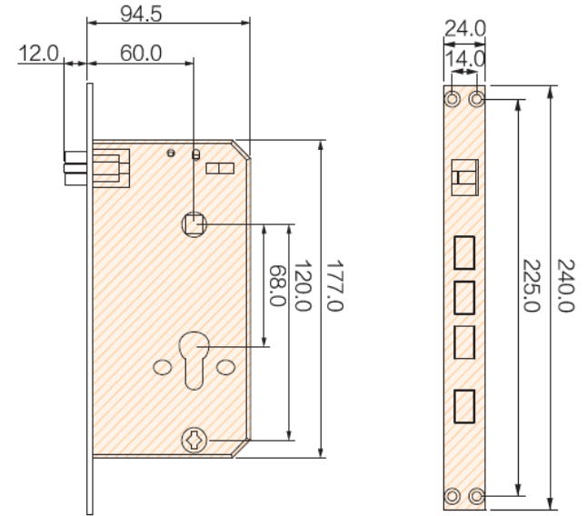
Lock Body(Unit: mm)
